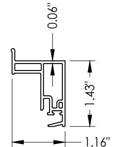
4 LOCK RAIL
