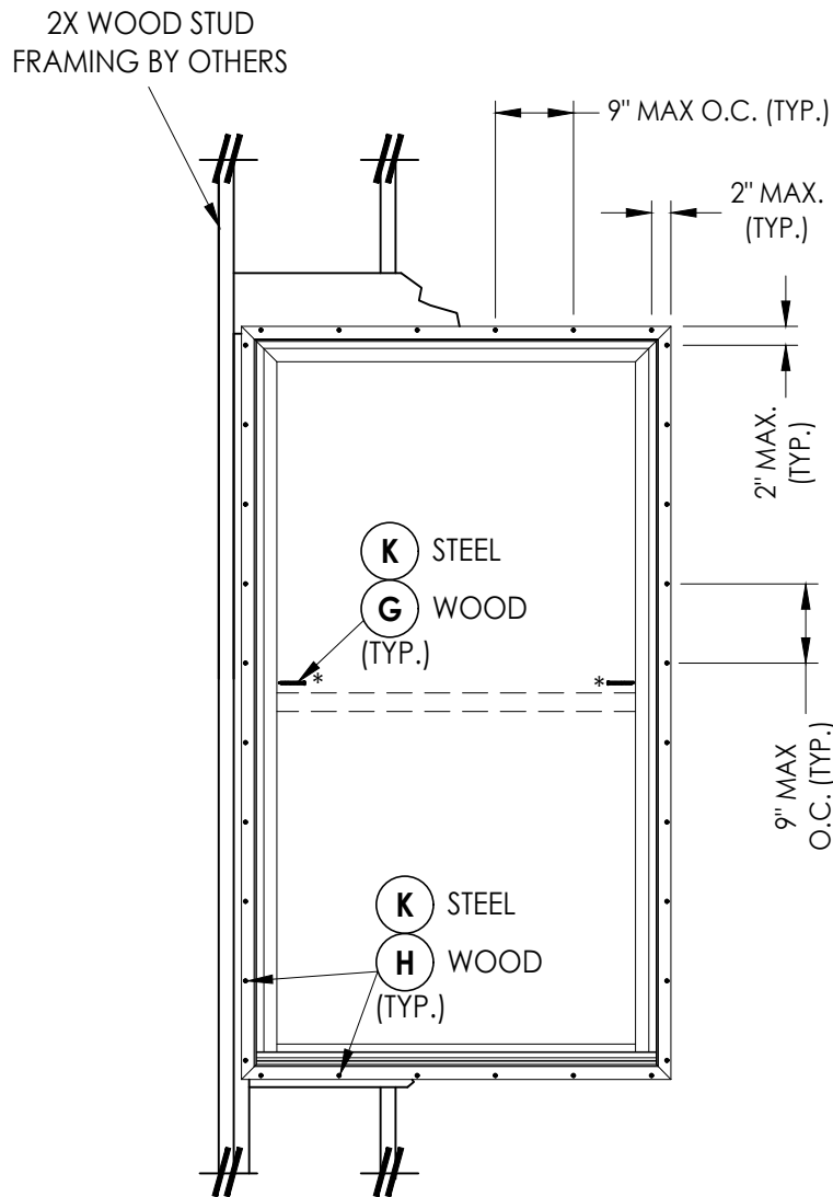
FRAME ANCHORING Stud Construction
