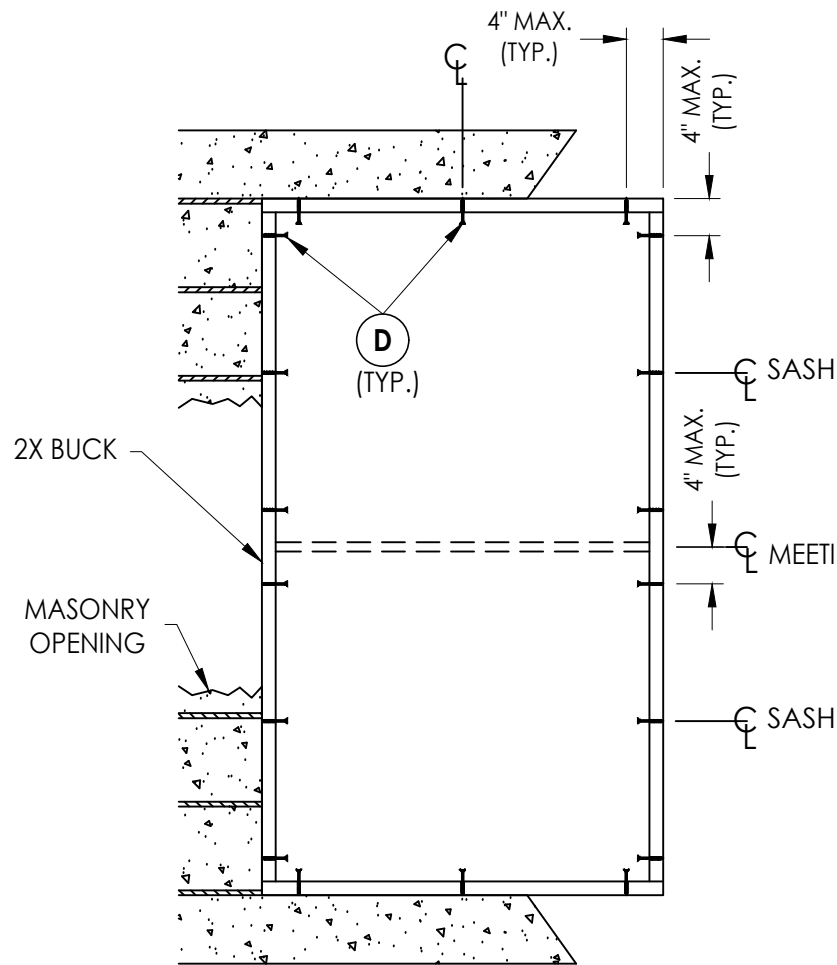
BUCK ANCHORING
