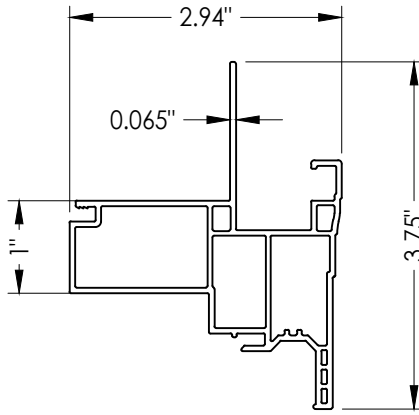
1 FRAME HEAD
