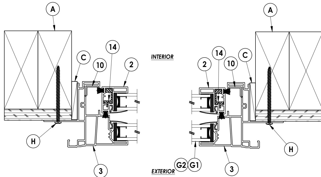
1 HORIZONTAL CROSS SECTION 3 Stud Construction
